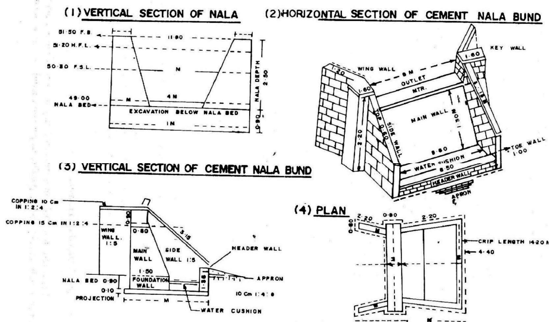
Fig 8.13 Design Aspects of a Cement Nalah Bund
