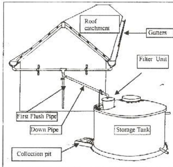
Fig 9.1 A Typical Rainwater Harvesting System
