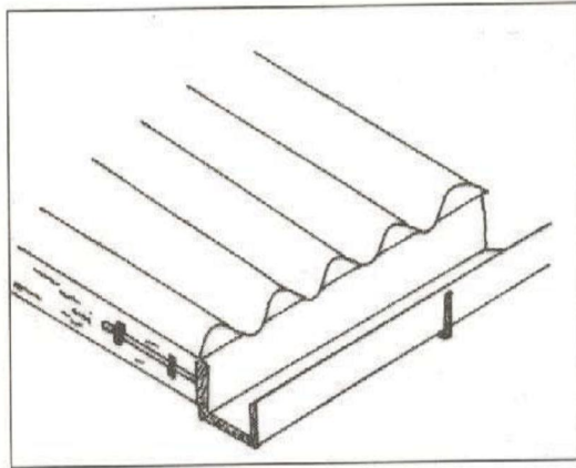
Fig. 9.2 Rectangular Gutter
