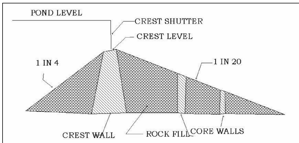
Fig. 8.17(b) A Typical Rock-filled Weir with Sloping Aprons.
