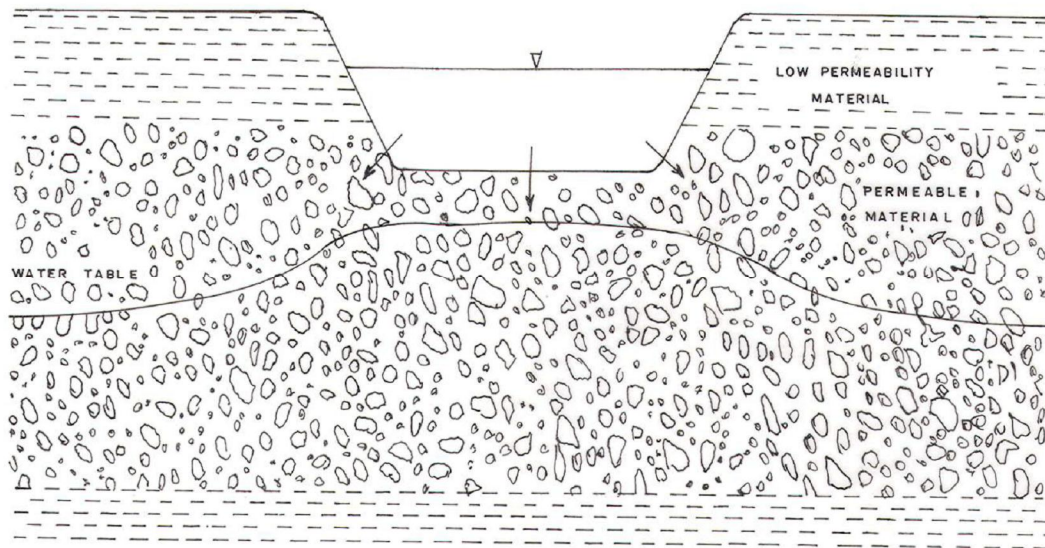
Fig.8.24 Schematics of a Recharge Pit.
