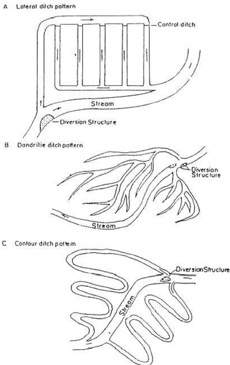
Fig 8.9 (a) Schematics of a Typical Ditch and Furrows Recharge System
