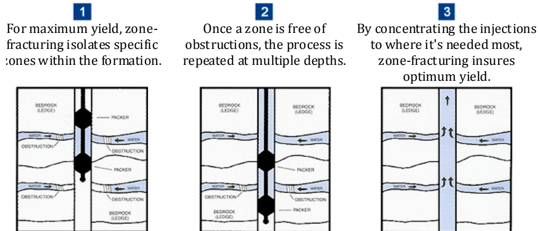
Fig 8.29 b Diagram showing packer arrangement for Multiple fracture system
