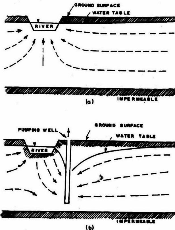
Fig.8.27 Principle of Induced Recharge through Pumping of Wells near a Stream a) Natural Flow Pattern b) Change in Flow Pattern Due to Pumping.
