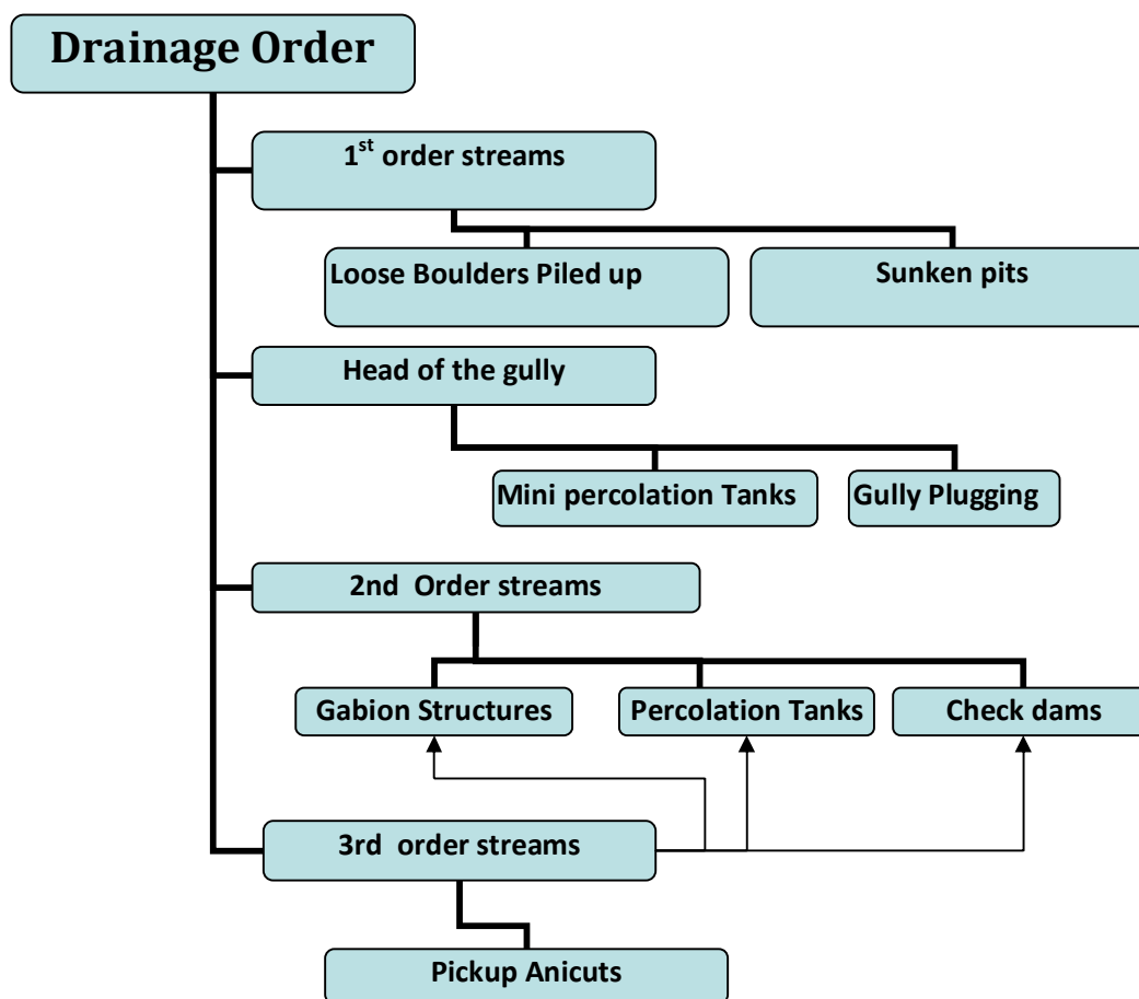
Fig 8.3 Decision support model for selection of Sustainability structures based on drainage order.
