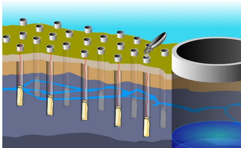
Fig 8.28 Diagram showing preparations for Borewell Blasting
