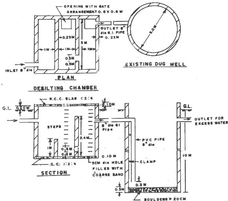
Fig 8.23 Schematics of a Typical System for Artificial Recharge through Dug Well.
