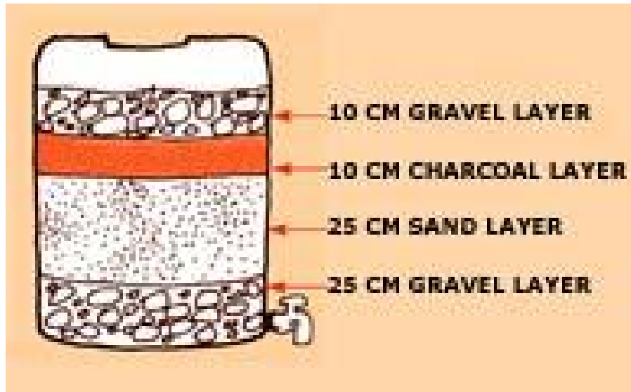
Fig 9.7 Charcoal Water Filter Source: A water harvesting manual for urban areas
