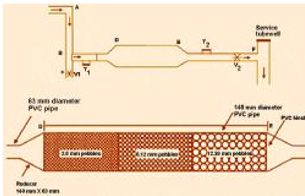
Fig 9.9 PVC Tube Filter Source: A water harvesting manual for urban areas
