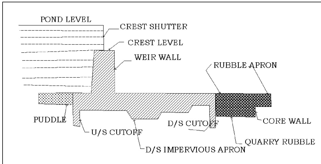
Fig. 8.17(a) A Typical Masonry Tank Weir with a Vertical Drop.
