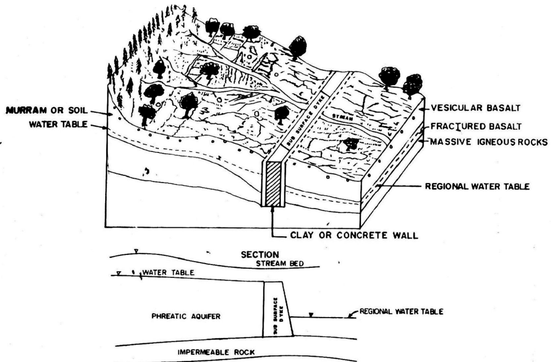
8.30 a Showing the three dimensional block diagram for a Sub-Surface Dyke
