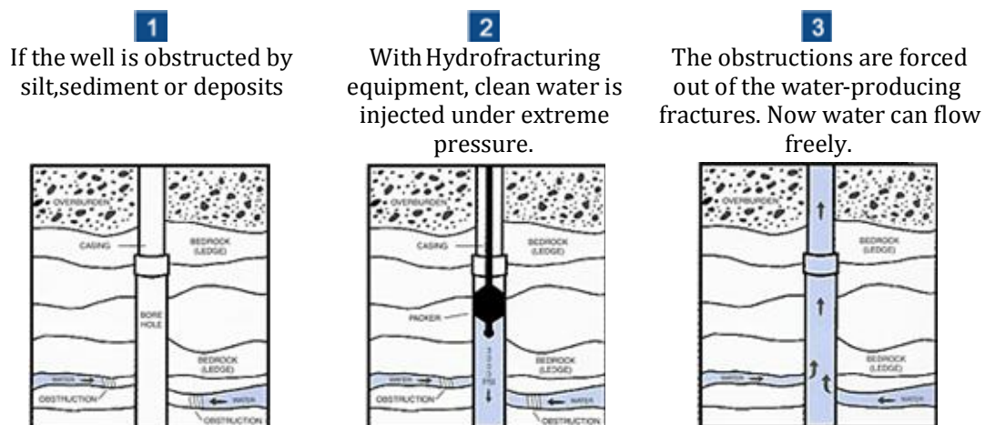
Fig 8.29 a Diagram showing packer arrangement for a clogged borewell
