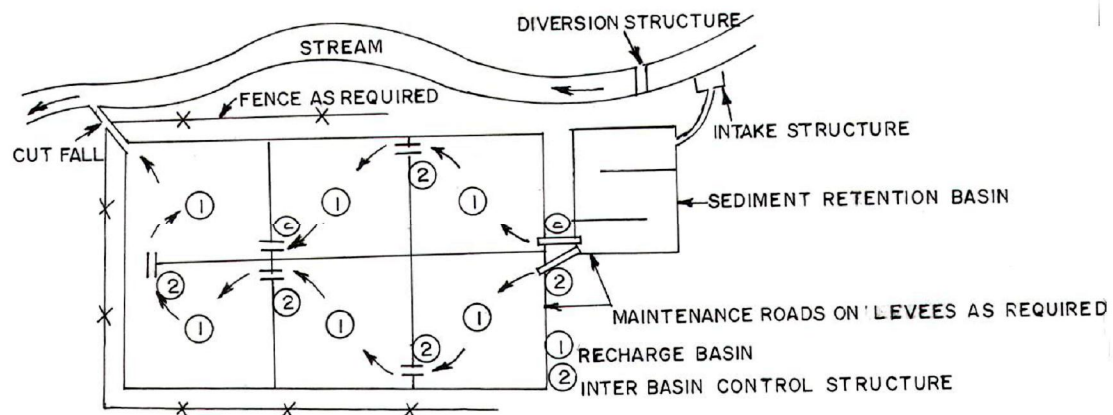
Fig 8.10 Schematics of a Typical Recharge Basin
