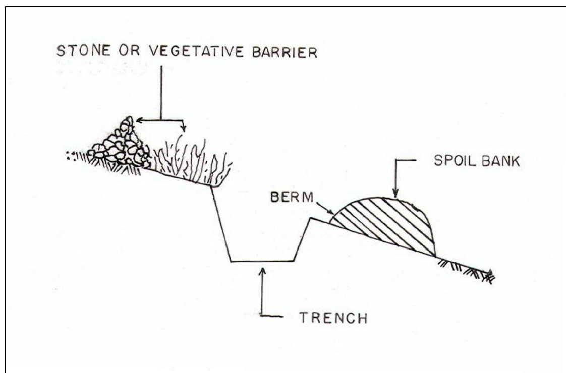
Fig 8.12 Schematics of a Contour Trench
