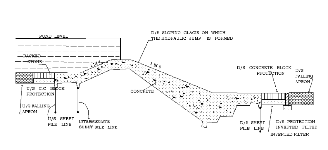
Fig. 8.17(c) Typical Cross-section of a Modern Concrete Weir with Permeable Foundation.
