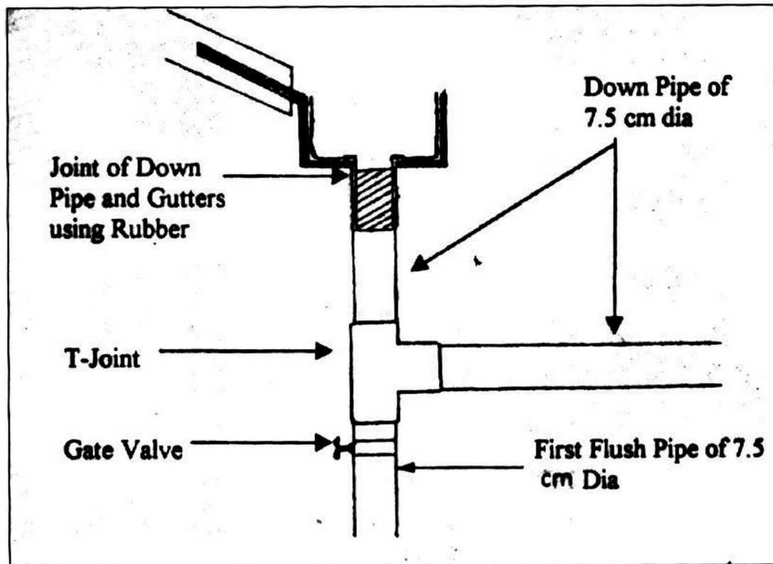
Fig 9.4 Downtake Pipe
