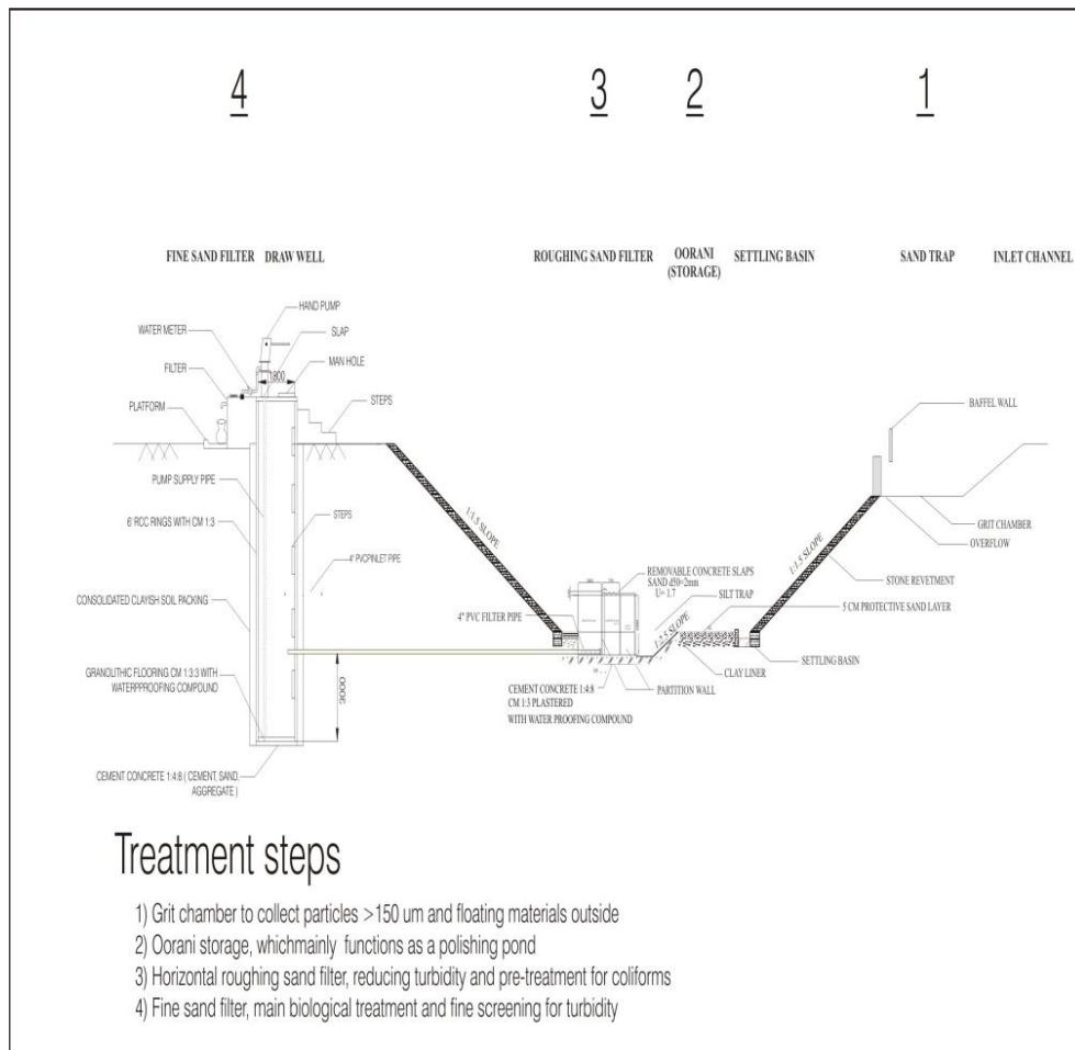
Fig 8.18 Typical Section of an Oorani
